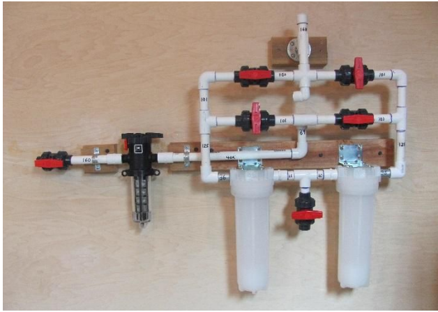
BACKFLUSH LEFT FILTER POSITION
